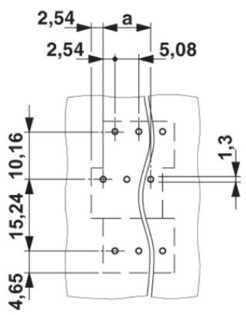
Drilling diagram
